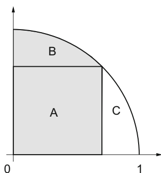
Fig. 8.6 Left: The shaded area is expressed as an integral in Example 8.7. Right: output from Simpson's rule
