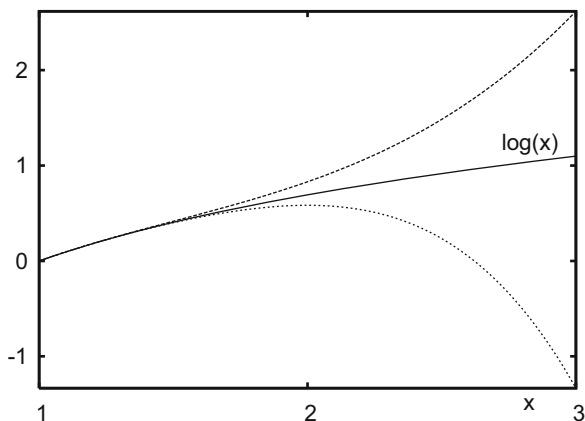
Fig. 4.16 Taylor's inequality for \log x as in Example 4.16
