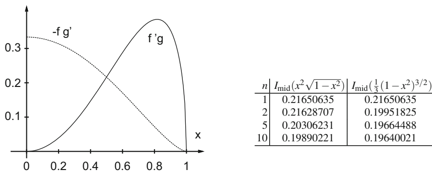
Fig. 7.1 Left: Graphs of the integrands f'(x)g(x) = x^2\sqrt{1-x^2} and -f(x)g'(x) = \frac{1}{3}(1-x^2)^{3/2} in Eq. (7.6). Right: Approximate integrals using values at the midpoints of n subintervals
