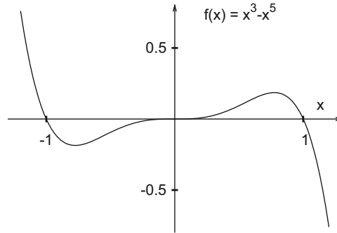
Fig. 4.11 A local maximum and a local minimum, in Example 4.13
