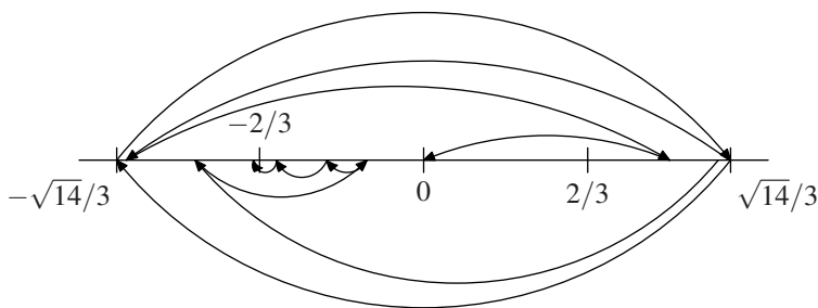
FIG. 11.5 Phase portrait of Tx = 1.8(x - x^3)
