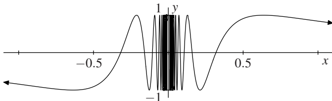
FIG. 5.3 A partial graph of \sin(1/x) .
