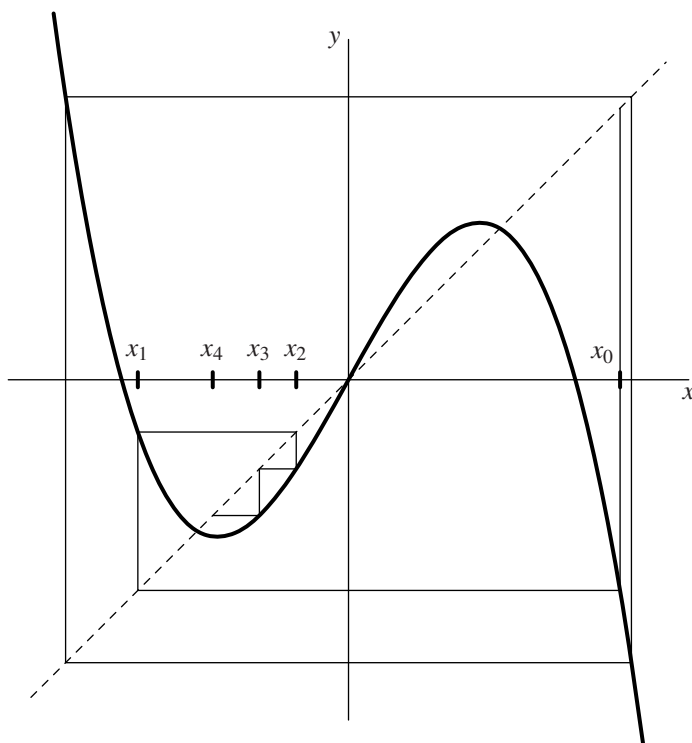
FIG. 11.4 Graph of Tx = 1.8(x - x^3) showing period-2 orbit and a nearby orbit.
