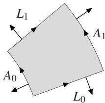
FIG. 13.1 The region R with boundary and outward normal vectors.
