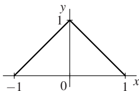
FIG. 15.5 The graph of the hat function h .
