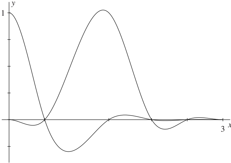
FIG. 10.7 Graphs of c_0 and c_2 for \Delta = \{0, .5, 1.4, 2, 2.5, 3\} .
