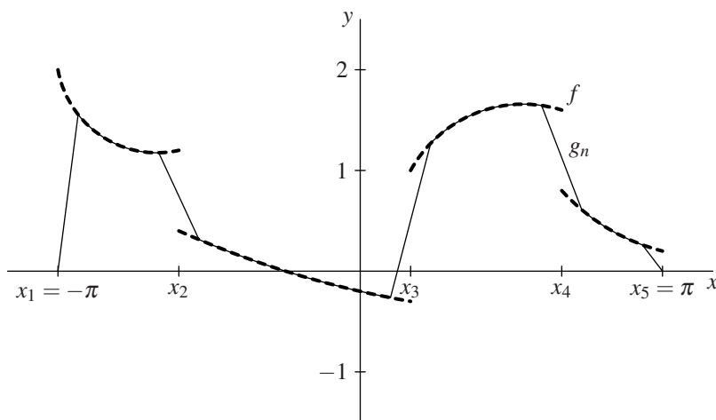
FIG. 14.5 Piecewise continuous f with continuous approximation g_n .
