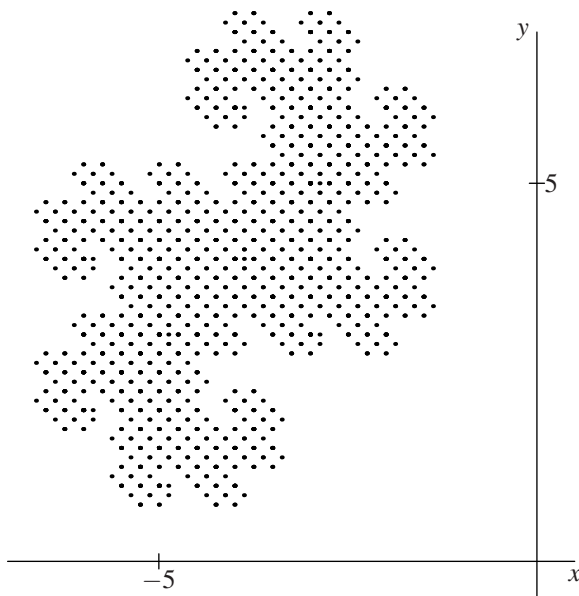
FIG. 11.12 Pointillist picture of the 'twin dragon' set.
