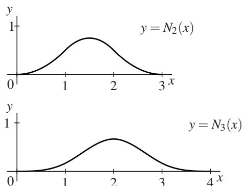
FIG. 15.7 The graphs of N_2 and N_3 .
