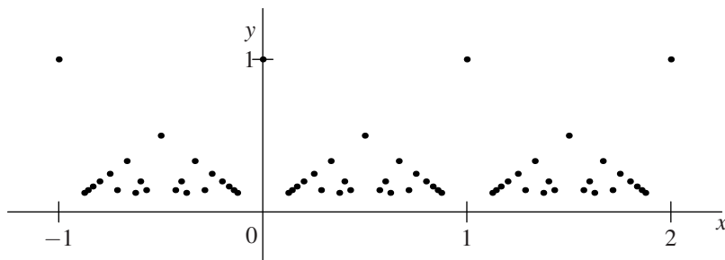
FIG. 5.4 Partial graph of function f(p/q) = 1/q .
