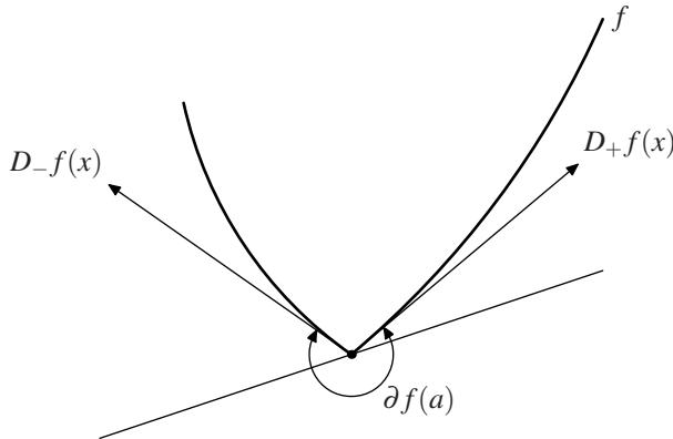
FIG. 16.5 The subdifferential and a tangent line at a nonsmooth point.
