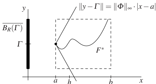
FIG. 12.2 Schematic setup for Local Picard Theorem.
