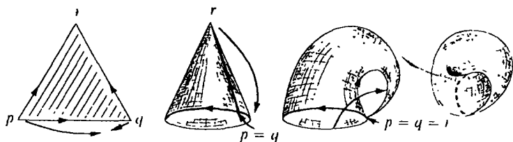
Figure I-6. The dunce cap
