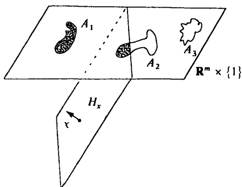
Figure IV-13. Ham sandwich
