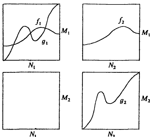
Figure VI-11. Coincidence doubling.
