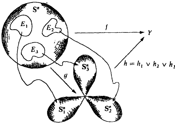
Figure IV-4. Setup for Theorem 7.4.
