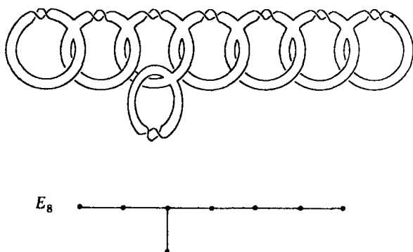
Figure VI-13. The Milnor plumbing.
