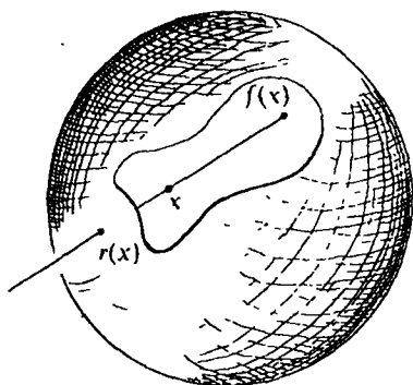
Figure 11-9. Retraction of disk.
