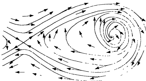
Figure U-6 Vector field and flow
