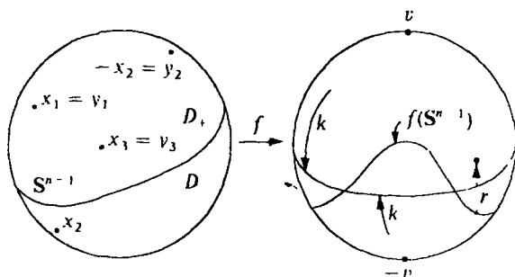
Figure IV-14. Proof of Theorem 20.6
