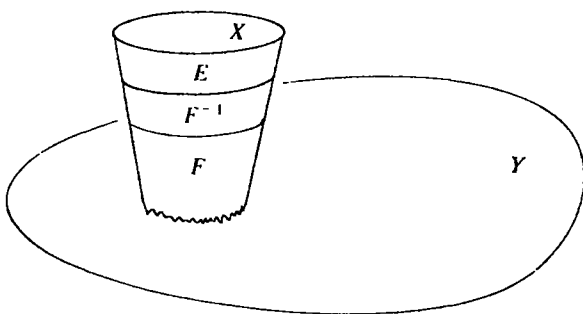
Figure I-5. Deformation of a mapping cylinder.
