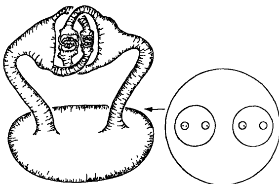
Figure IV-9. The Alexander horned disk.
