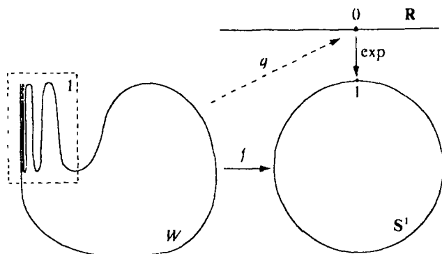
Figure III-6. Discontinuous lifting
