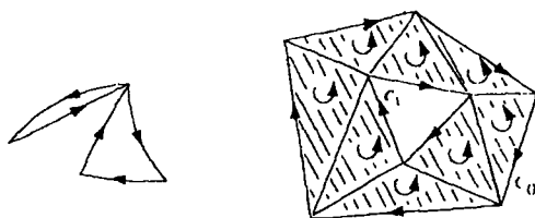
Figure IV-1 Examples of chains
