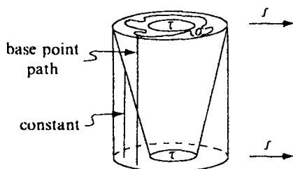
Figure VII-10. Stage 2 homotopy.
