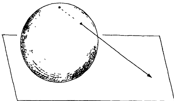
Figure II-2 Stereographic projection
