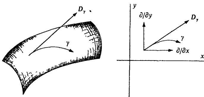
Figure II-4. Tangent vectors.
