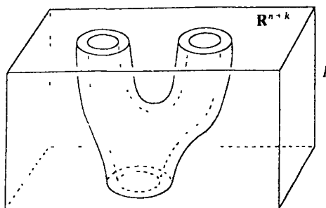
Figure II-14 A cobordism
