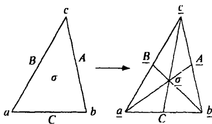
Figure IV-7 Barycentric subdivision
