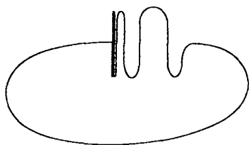
Figure VII-2 A pseudo-circle.
