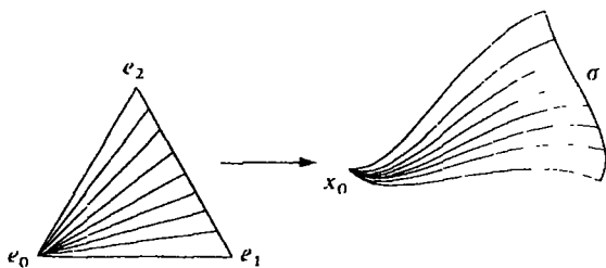
Figure IV-6. A chain homotopy.
