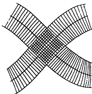
Figure VI-12. Simple plumbing.
