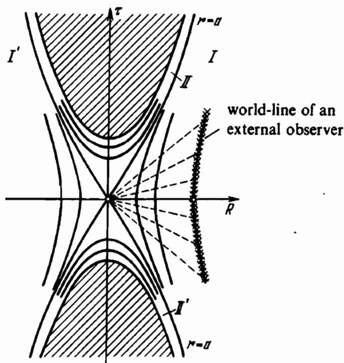
Figure 115. The (R, \tau) -plane. The “meaningless” region r \leq 0 is shaded. The solid curves represent the level curves r(R, \tau) = \text{const.} , and the dotted lines the level curves t(R, \tau) = \text{const.} (Here t is the time co-ordinate in the Schwarzschild region r > a ; see (6).) At r = a we have |t| = \infty except for the origin R = \tau = 0 , where the time is undefinable since all of the level curves t = \text{const.} converge there. At that point we have \partial r / \partial \tau = \partial r / \partial R = 0 ; it is in fact a saddle point. On the curves r = a we have \langle \nabla r, \nabla r \rangle = 0 . The regions I and I' are isometric (under the map R \leftrightarrow -R ), as are the regions II and II' ( \tau \leftrightarrow -\tau ).
