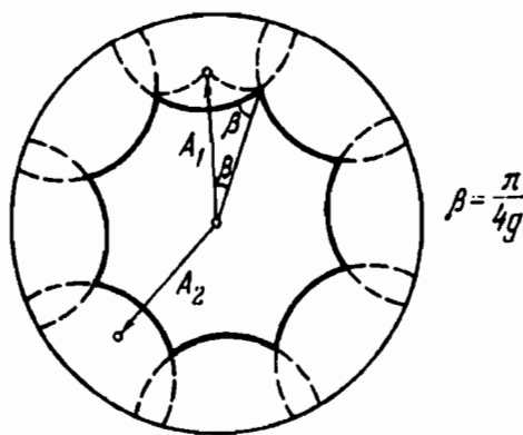
Figure 76. The transformations A_1 and A_2 translate the centre of the octagon to the positions indicated by the arrows.
