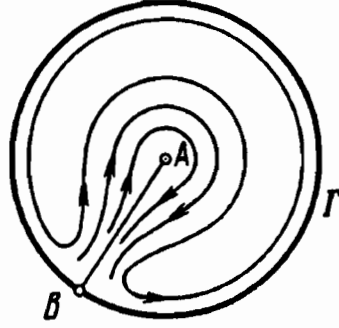
Figure 103. The points A and B are singular, with the point B on the boundary \Gamma a saddle; on the segment BA no time-direction is definable.
