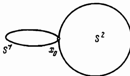
Figure 56. The bouquet S^1 \vee S^2 .
