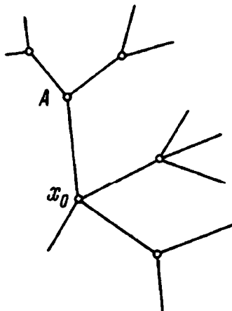
Figure 54. (Part of) a tree A \sim x_0 .
