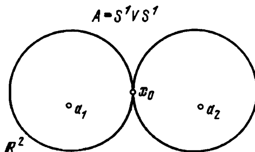
Figure 55. A bouquet of two circles.
