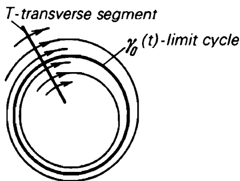
Figure 104. The Poincaré function f: T \rightarrow T is defined for each \tau \in T in terms of the trajectory \gamma starting at \gamma(0) = \tau : we set f(\tau) = \gamma(t) , where \gamma(t) \in T is the first point where the curve \gamma again meets T . In particular if \tau \in T is on the limit cycle \gamma_0 , then f(\tau) = \tau .
