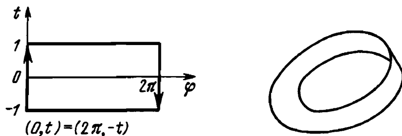
Figure 47. The Möbius strip in \mathbb{R}^3 (a “one-sided surface”).
