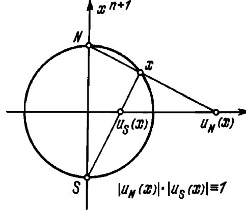
Figure 1. Local co-ordinates on the sphere via stereographic projections.
