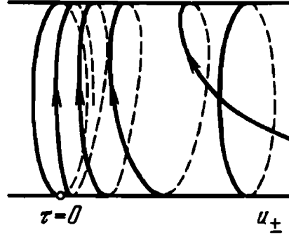
Figure 120. The (u, v) -cylinder, showing a curve x = \ln u_- + v_- = \text{const.}
