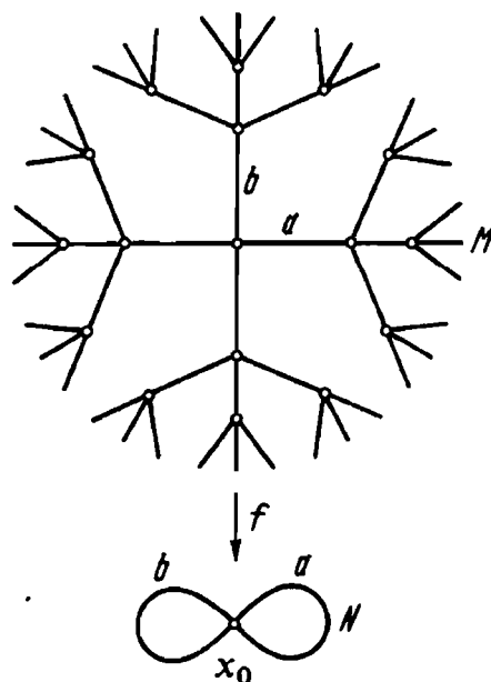
Figure 59. Here M is an infinite tree of “crosses”, i.e. with exactly 4 edges incident with each vertex. Being a tree, M has no “cycles”, and is therefore contractible to a point.
