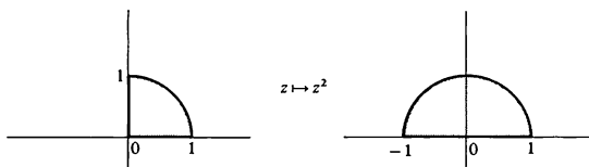
Isomorphism between quarter disc and half disc
