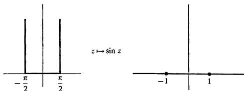
Upper half strip with upper half plane
