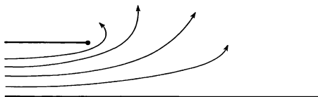
Flow lines in the (u, v) -plane
