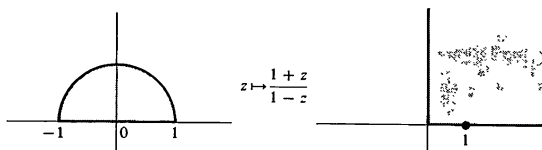
Upper half disc with first quadrant
