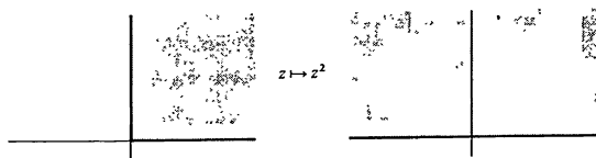
Isomorphism between first quadrant and upper half plane
